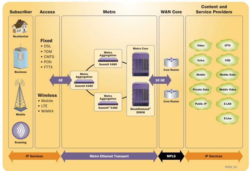
Figure 13: Summit X480 in a Carrier Ethernet Application
