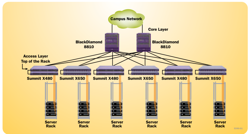
Figure 10: Top-of-Rack Architecture with Hybrid Deployment
