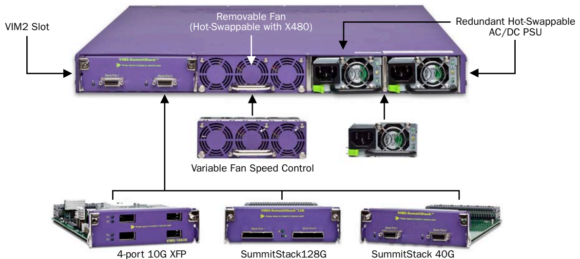
Figure 6: Summit X480 High Availability Design
