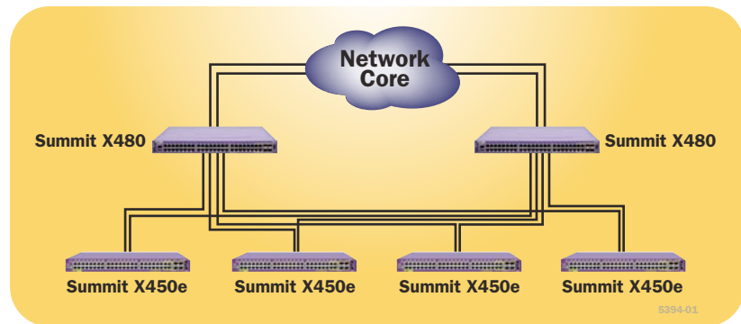
Figure 12: Summit X480 as an Aggregation Switch in a Three-Tier Network
