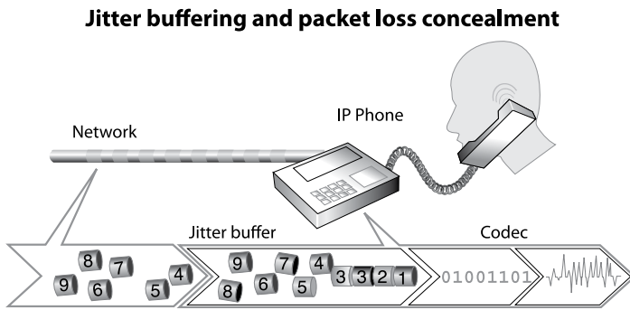
VoIP packets can arrive at the receiving phone out of sequence, late, early, or not at all. IP phones use a jitter buffer to reconstruct the packet stream at the receiving end, duplicating missing packets or filling in with white comfort noise when necessary.
